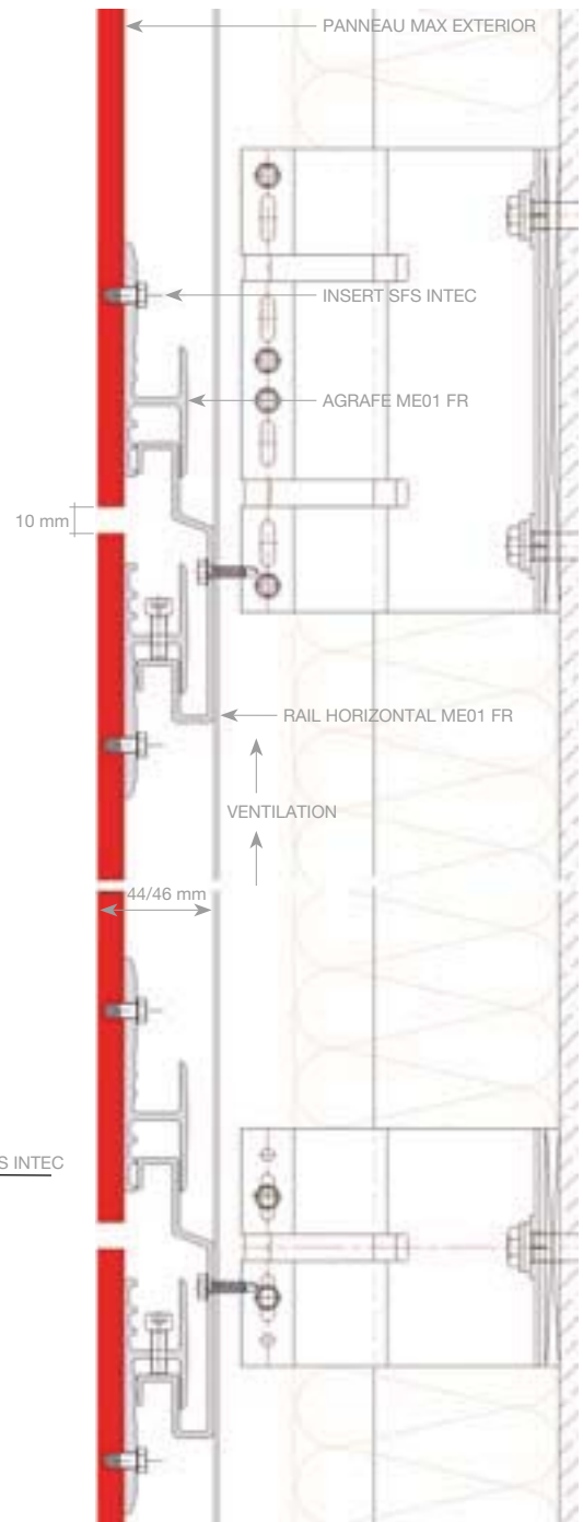
COUPE VERTICALE JOINT HORIZONTAL
